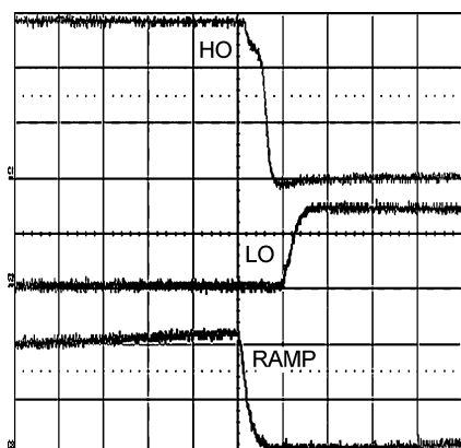
Figure 11. Adaptive Delays
