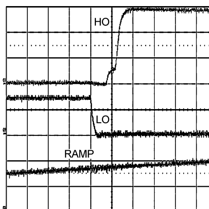
Figure 10. Typical Waveforms
